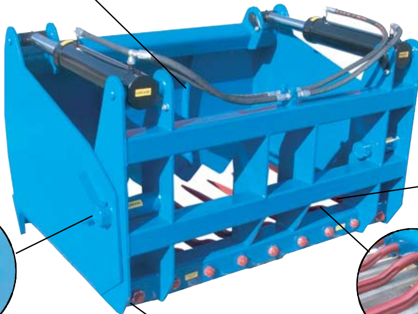
main beam wear plates and closed off side tine reinforcement
