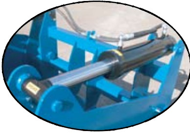
Heavy duty hydraulic cylinders for reduced power requirements
